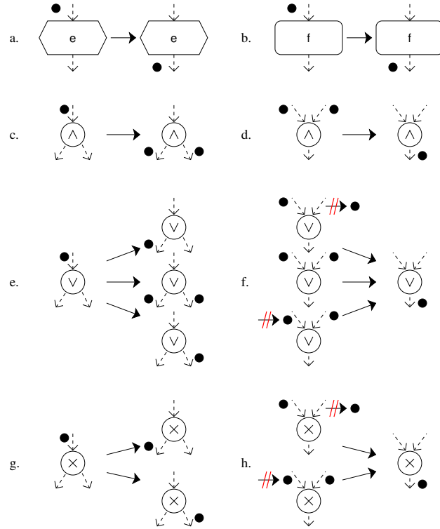
Figure 2: The transition relations for the different nodes
