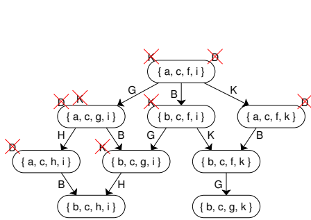
Figure 11: Adding non-local connector
