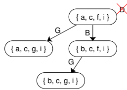
Figure 13: Adding transitions for connector G
