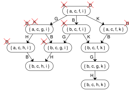
Figure 12: Local forward construction
