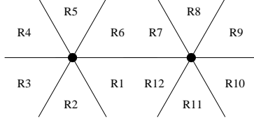
Figure 2: Partitioning of the two-dimensional space into regions R_1, \dots, R_{12}
